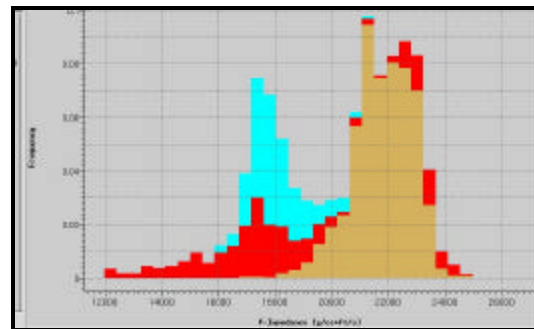
Figure 2 Eastern Province Lithofacies Stacked Histogram: frequency of occurrence of impedance values of the three eastern province lithofacies
