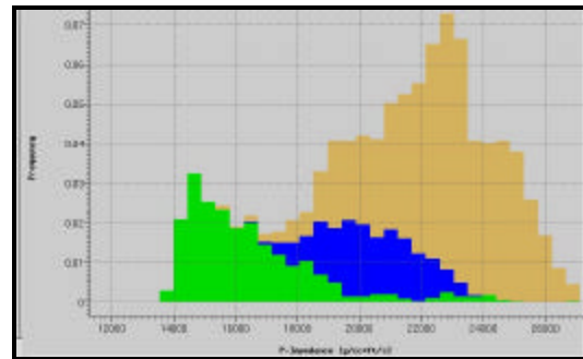
Figure 1 Western Province Lithofacies Stacked Histogram: frequency of occurrence of impedance values of the three western province lithofacies
