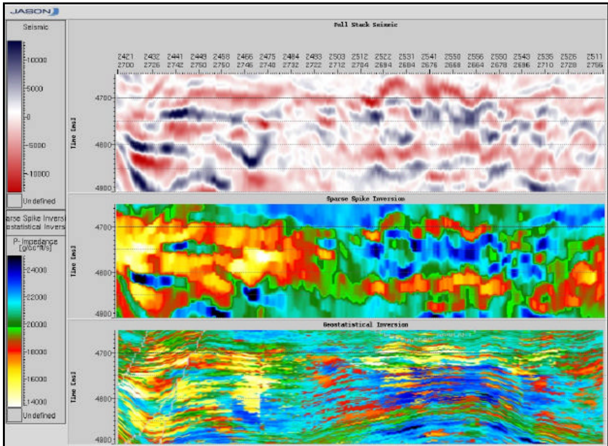
Figure 3. Time sections flattened on the B20 horizon. The top panel is the full seismic. The center panel is the constrained sparse spike inversion of the full seismic. The lower panel is the acoustic impedance from the selected geostatistical inversion realization .
